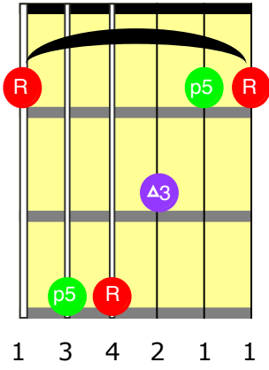
Root on 6
