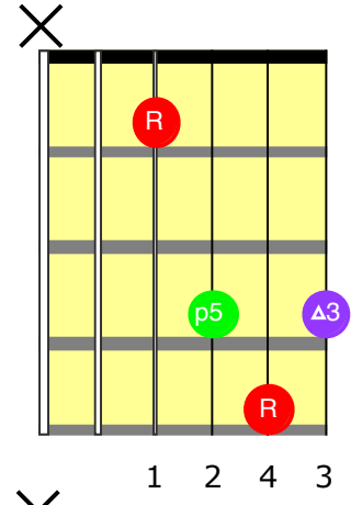
Root on 4
