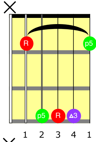
Root on 5
